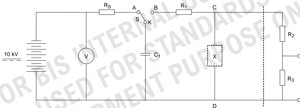
Figure 4 – Test hook
