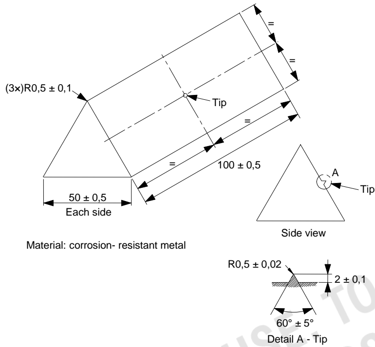
Figure 14 – Mandrel
