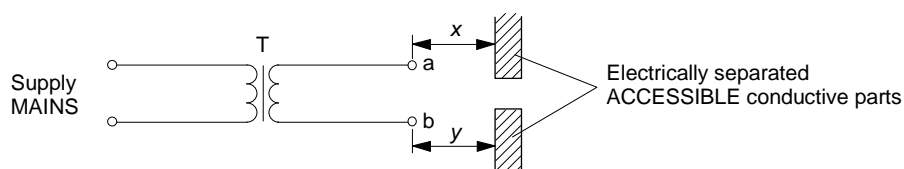
Figure 1 – Test circuit for fault conditions
