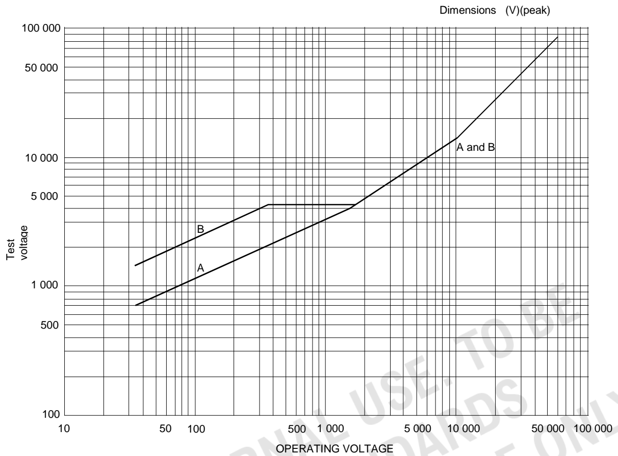
Figure 7 – Test voltages
