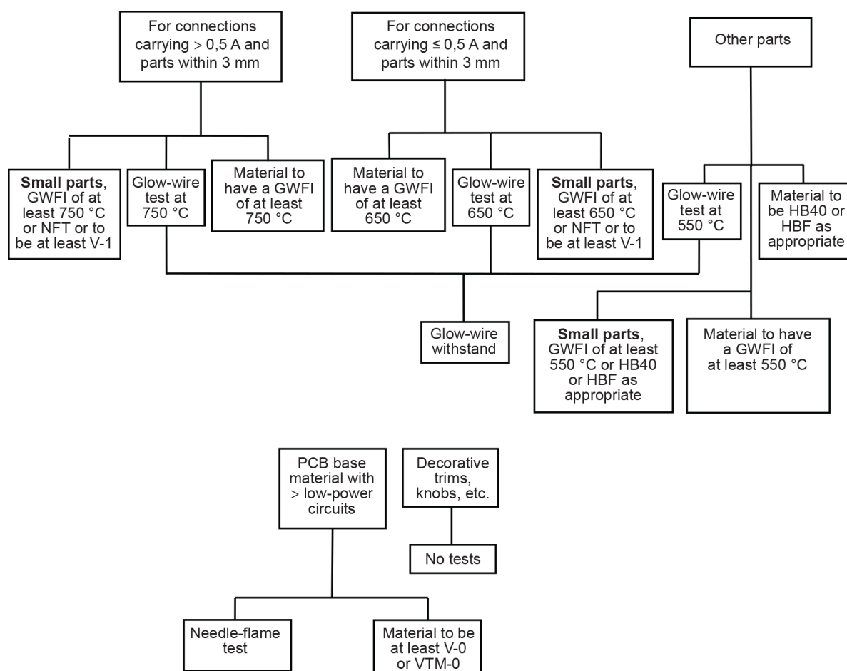
Figure O.2 – Selection and sequence of tests for resistance to fire in hand-held appliances
