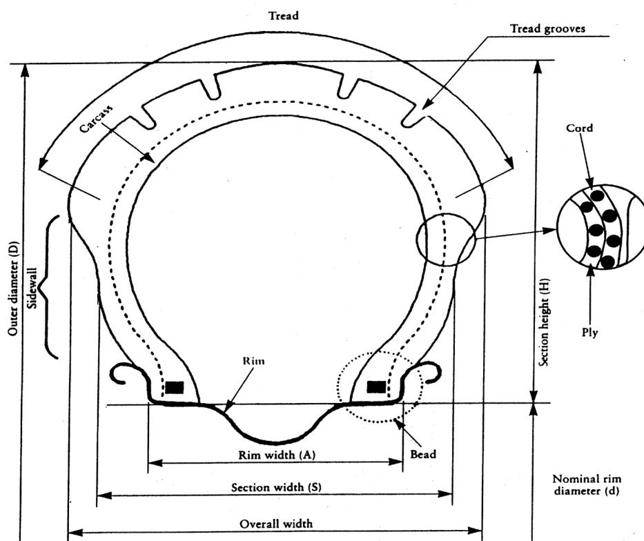
FIG.1 NOMENCLATURE OF TYRE
